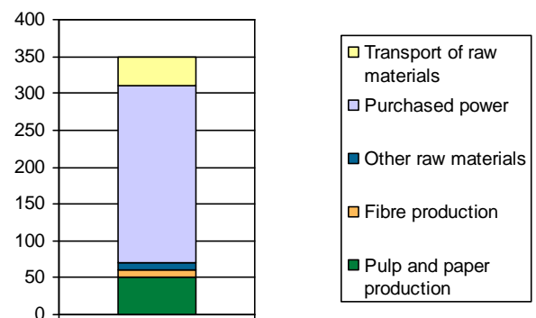
Carbon footprint of Shotton PM 2 [kg fossil CO 2 per tonne of paper]
