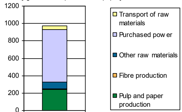
Carbon footprint of Schongau PM 9 [kg fossil CO 2 per tonne of paper]
