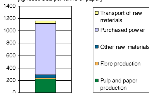
Carbon footprint of Schongau PM 7
