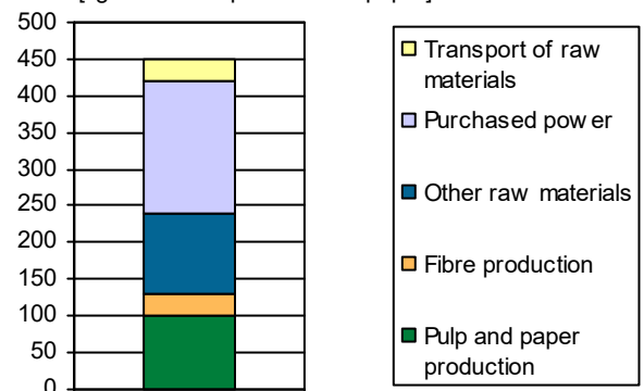
Carbon footprint of Rauma PM 1 [kg fossil CO 2 per tonne of paper]
