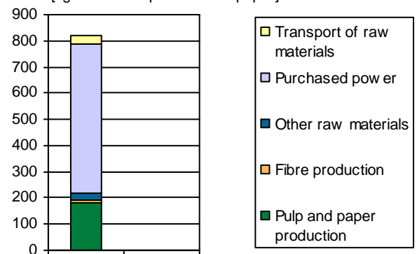
Carbon footprint of Ettringen PM 5 [kg fossil CO 2 per tonne of paper]
