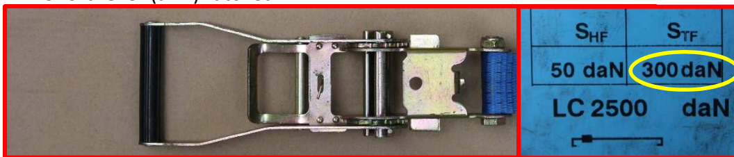
Short-lever (arm) ratchet
